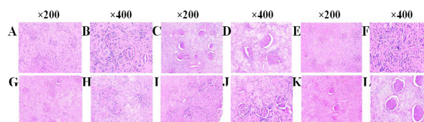
Fig. 5. Effect of SBG on histological structure of rats in ( \times 200 , \times 400 ). A, B: control; C, D: Model group; E, F: Positive drug group; G, H: SBG-H dose group; I, J: SBG-M dose group; K, L: SBG-L dose group. Stain: H & E. Magnification: A, C, E, G, I, K= 200X; B, D, F, H, J, L=400X.
