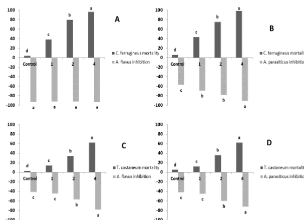
Fig. 3. Beetles' mortality and subsequent fungal infection inhibition at different concentrations of imidacloprid: (A) C. ferrugineus vs A. flavus , (B) C. ferrugineus vs A. parasiticus , (C) T. castaneum vs A. flavus , (D) T. castaneum vs A. parasiticus . In all cases, p < 0.01 .
