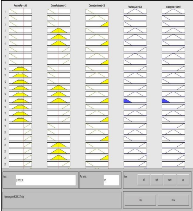
Fig. 4: Rule Viewer for 5CSMFC
