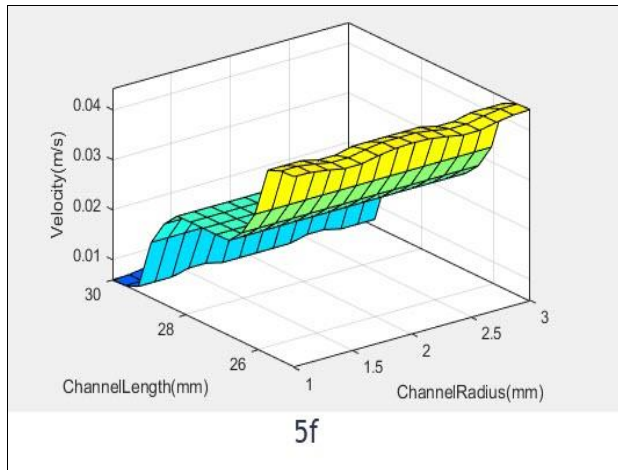
Fig. 5a, b, c, d, e, & f: 3D graphs of Fuzzy simulation, 5a (flow rate vs pressure and channel radius), 5b (flow rate vs pressure and channel length) and 5c (flow rate vs channel length and channel radius), 5d (velocity pressure and channel radius), 5e (velocity vs pressure and channel length) and 5f (velocity vs channel length and channel radius).
