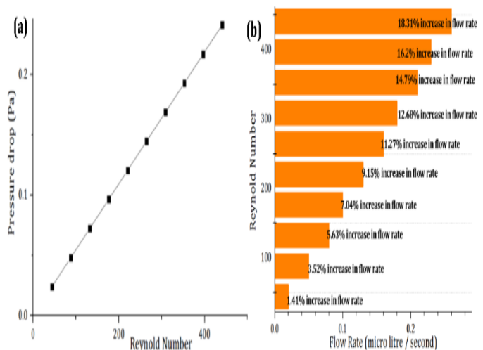
Fig. 2a & b: (a) graph between Reynolds number and pressure drop, (b) bar graph between Reynolds number and flow rate.
