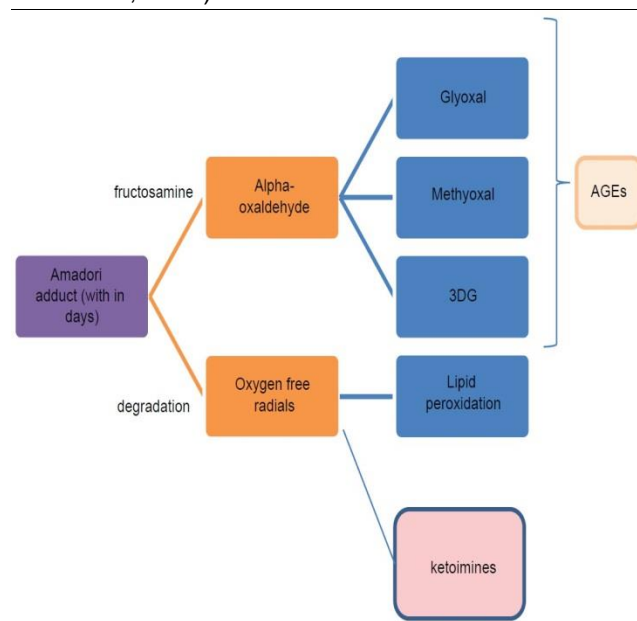
Fig. 1b: Amadori adduct outcomes
