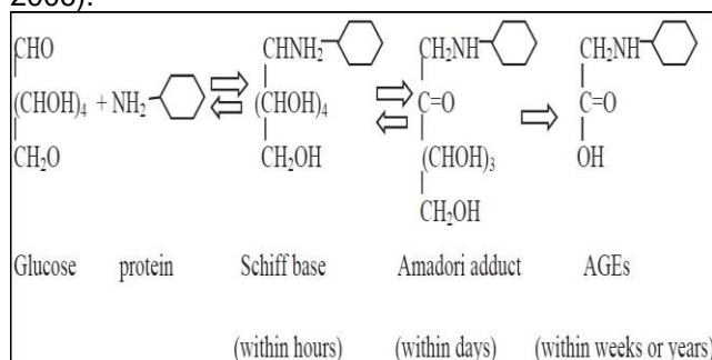
Fig.1a: Production of early and late non enzymatic glycation products (Neelofar & Ahmad, 2015)
