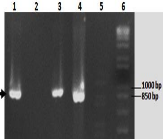
Fig. 2: Amplification of complete ORF3 (902 bp, arrow head) from Pak naHEV strains bile samples (2% Agarose Gel). Lane 1 = PT12B, lane 2 = PT14B, lane 3 = PT16B, lane 4 = positive control, lane 5 = negative control, lane 6 = 1 kb plus DNA marker
