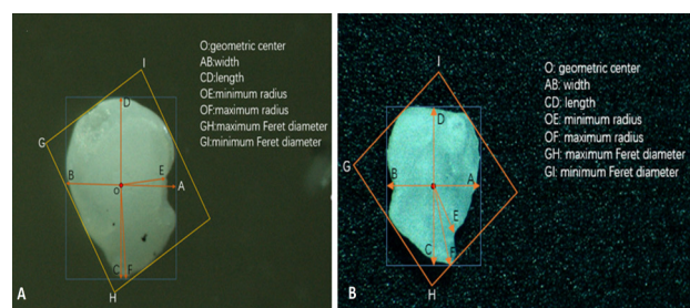
Fig. 1. Measurement illustration of sagitta in Sc. grahami (A), and Sp. sinensis (B).
