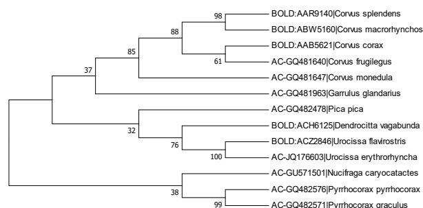
Fig. 2. The bootstrap consensus tree of thirteen nucleotide sequences of taxa of family Corvidae reported from Pakistan inferred by the Neighbor- Joining method using 1000 replicates to show their evolutionary relationships with final dataset of total 563 positions by MEGA7. The percentage of replicate trees in which the associated taxa clustered together in the bootstrap test (1000 replicates) are shown next to the branches.
