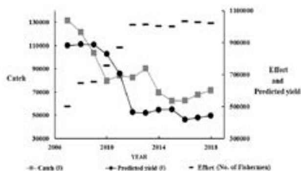
Fig. 1. Catch, effort and predicted yield for T. lepturus .
