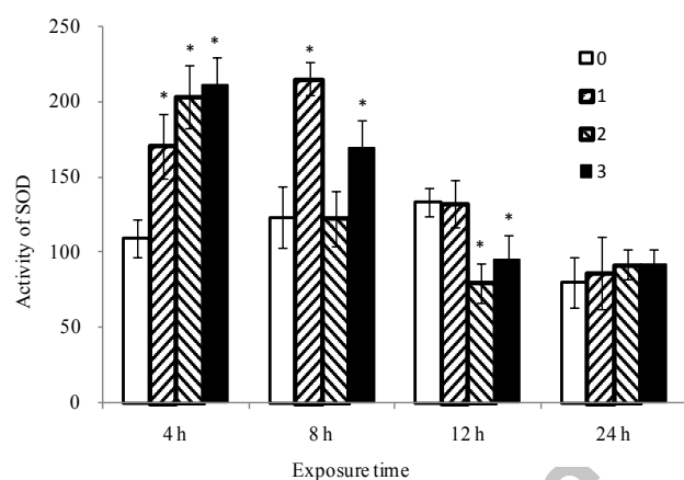
Fig. 2. Activity of super oxide dismutase in the fat bodies of A. pernyi exposed to different concentration of uranyl acetate. The values represent mean \pm SE (n=3). For each experiment, samples were analyzed in triplicate. (0: Control; 1: 6.25 mM; 2: 12.5 mM; 3: 25 mM.).
