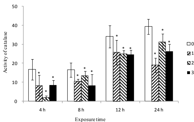
Fig. 4. Activity of catalase in the fat bodies of A. pernyi exposed to different concentration of uranyl acetate. The values represent mean \pm SE (n=3). For each experiment, samples were analyzed in triplicate. (0: Control; 1: 6.25 mM; 2: 12.5 mM; 3: 25 mM.).
