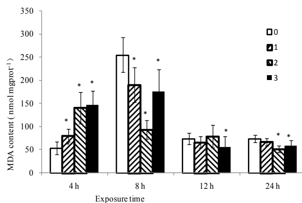
Fig. 1. MDA content in the fat bodies of A. pernyi exposed to different concentration of uranyl acetate. The values represent mean±SE (n=3). For each experiment, samples were analyzed in triplicate. (0, Control; 1, 6.25 mM; 2, 12.5 mM; 3, 25 mM.).
