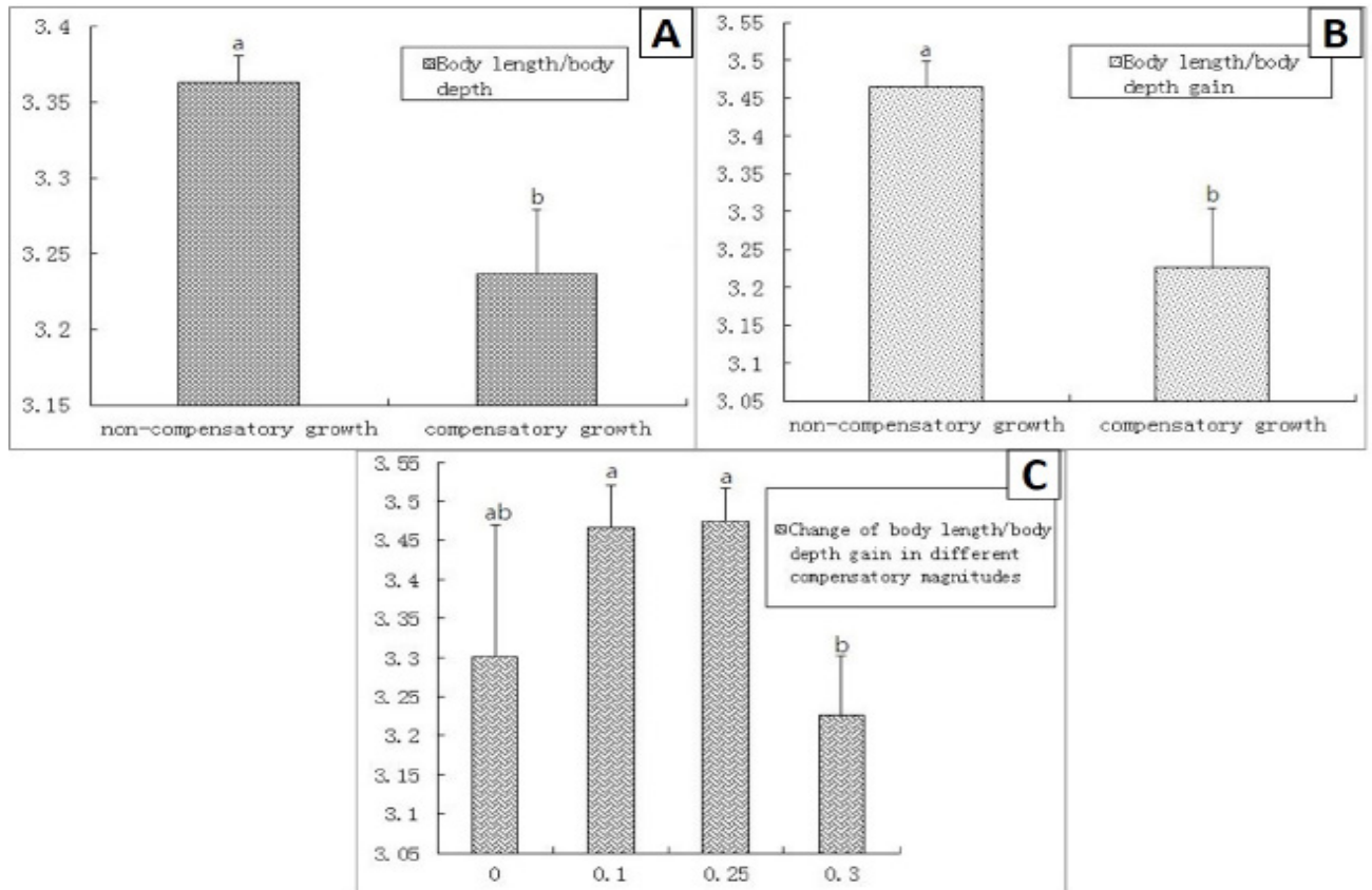
Supplementary Fig. S2. Magnitude of compensatory growth of the body length/body depth. A , compensatory growth effect on body length/body depth, non-compensatory growth group had the higher body length/body depth; B , compensatory growth effect on body length/body depth gain, non-compensatory growth group also had the higher body length/body depth gain; C , change of body length/body depth under different magnitude of catch-up growth. Both 0.1 and 0.25 levels make the body length/body depth gain bigger than the 0.3 level, while no different significant difference of such ratio was found between compensatory group and control group.
