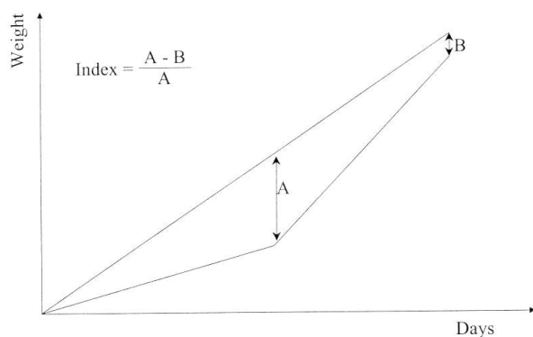
Supplementary Fig. S1. The compensatory index, a method to measure the catch-up growth: A is the difference of body weight during first growth stage (catch-up group influenced by restricted factor and control group with no influence by such factor), B is the difference of body weight during second growth stage where the catch-up group were feed as control group.
