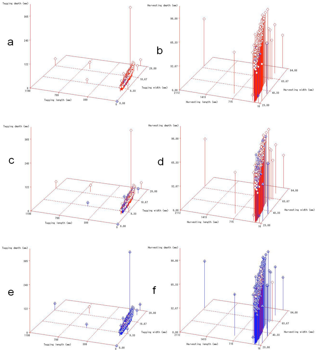
Supplementary Fig. S3. Different compensatory growth magnitude effect on body shape. a, c and e , 3D graphs for body length, body width, body depth on PIT tagging; b, d and f , 3D graphs for body length, body width, body depth on harvesting; a and b , 0.10 level for compensatory growth observed; c and d , 0.25 level for compensatory growth observed; e and f , 0.30 level for compensatory growth observed; red present non-compensatory growth, blue instead of catch-up growth. From the level 0.1 to level 0.3, body shape on both tagging and harvesting defined as the colour components showed that the compensatory growth observed were increased (with more expanded blue area).
