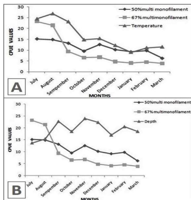
Fig. 1. Monthly CPUE values of mirror carp caught by multi-monofilament gillnets with different hanging ratios (0.5 and 0.67) depending on water temperature (A) and water depth (B).
