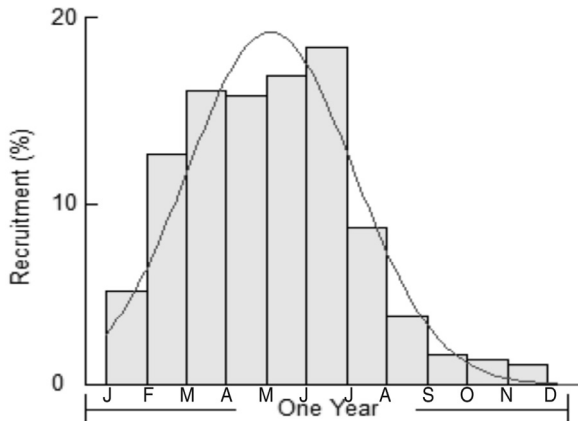
Fig. 6. The annual recruitment pattern of O. mykiss .
