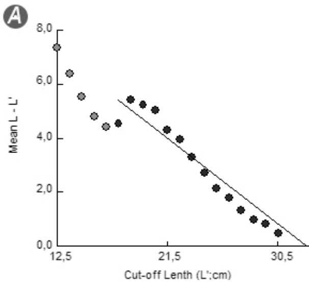
Fig. 4. Powell-Wetherall plot for (A) and Pseudo-Catch Curve (B) O. mykiss .
