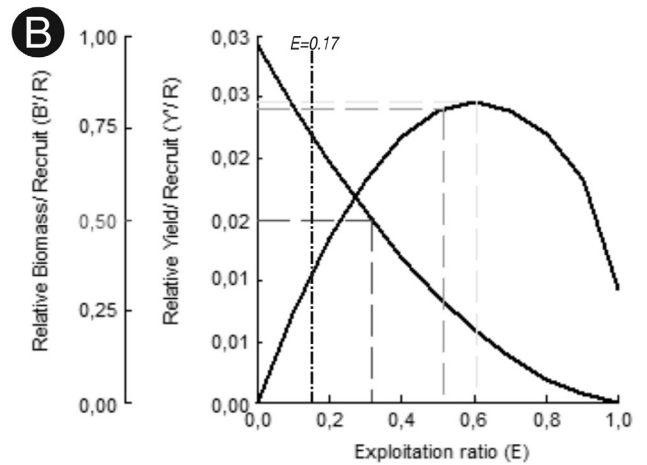
Fig. 9. Relative yield and biomass recruit of O. mykiss using selection Knife Edge selection procedure (A) and Ogive selection procedure (B).
