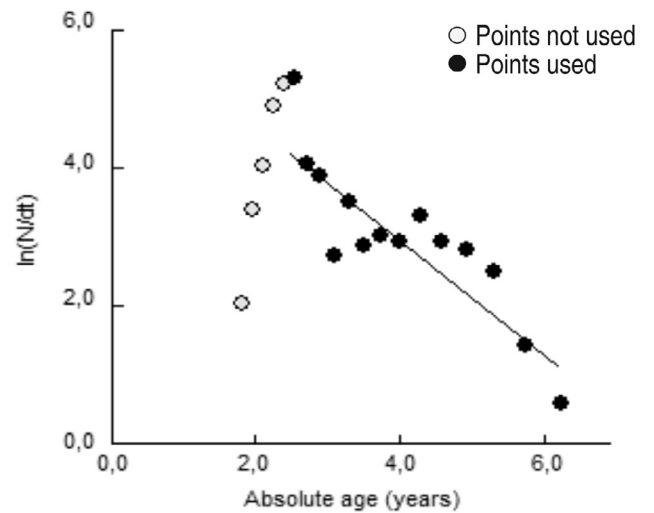
Fig. 8. Length-converted catch curve of O. mykiss .
