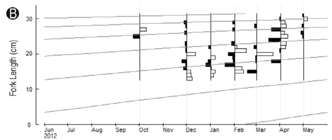
Fig. 5. von Bertalanffy growth curves of O. mykiss with normal length-frequency histogram (A) and restructured histogram (B).
