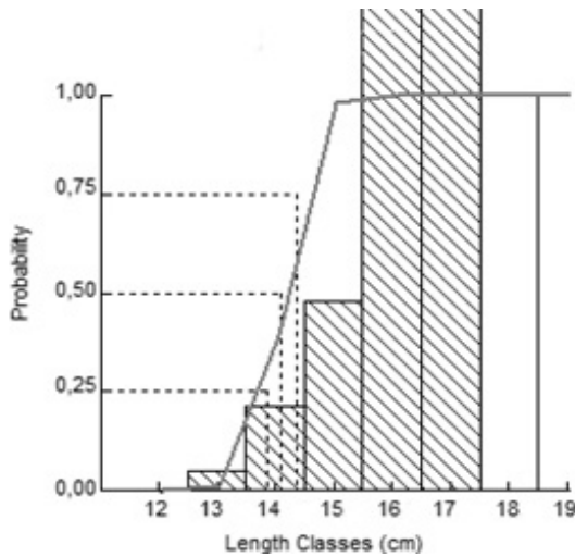
Fig. 7. Probability of capture analysis for O. mykiss .
