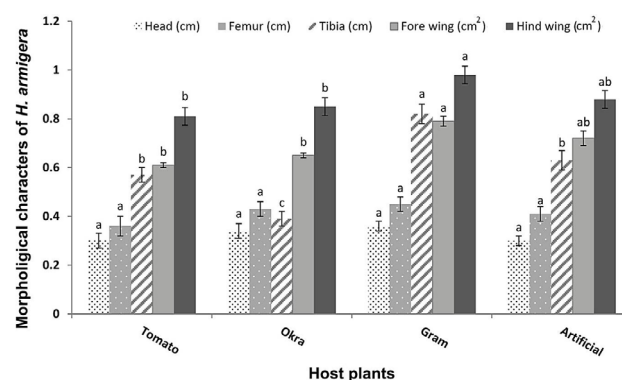
Fig. 3. Variations among morphological character measurements (cm 2 /cm) (Means \pm SE) of H. armigera adults in response to feeding on different host plants and artificial diet (Treatments showed significance only for tibia length and areas of fore wing and hind wing at P < 0.001 ).
