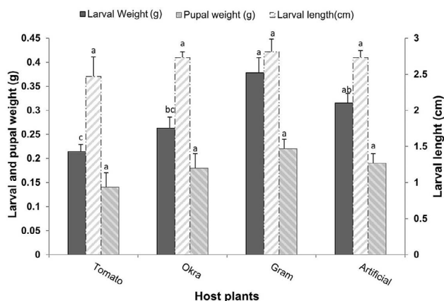
Fig. 1. Larval and Pupal weights and larval length (Means \pm SE) of H. armigera in response to feeding on different host plants and artificial diet, Pupal weight and larval length are not significant at P > 0.05 .
