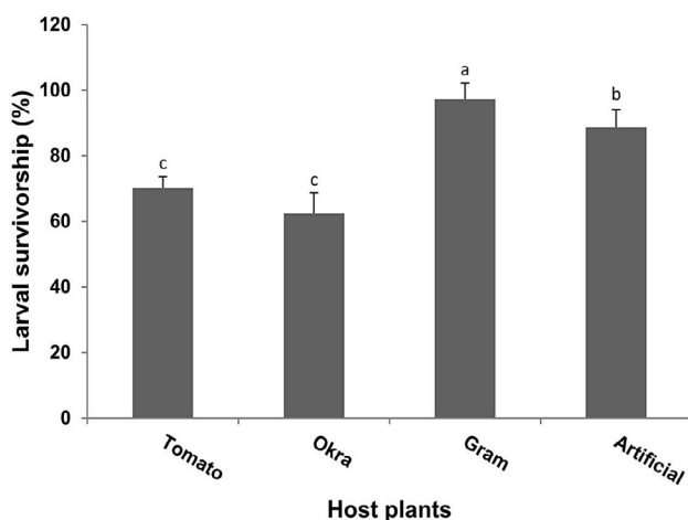
Fig. 2. Percent larval survivorship (Means \pm SE) of H. armigera in response to feeding on different host plants and artificial diet same letters representing the bars are not significant according to Tukey (HSD) test at P > 0.05 .
